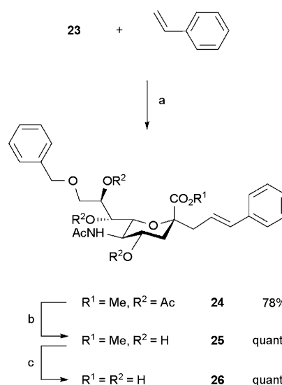
Scheme 5 a) catalyst 1 , CH 2 Cl 2 , reflux; b) NaOMe, MeOH, rt; c) 0.1 M NaOH, H 2 O, rt.
