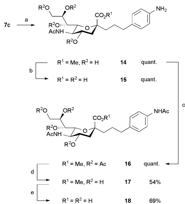
Scheme 3 a) H 2 , Pd/C, MeOH, rt; b) Et 3 N, H 2 O, rt; c) Ac 2 O, pyridine, rt; d) NaOMe, MeOH, rt; e) 0.1 M NaOH, H 2 O, rt.
