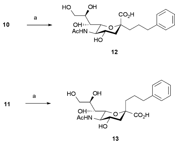
Scheme 2 a) 0.1 M NaOH, H 2 O, rt.
