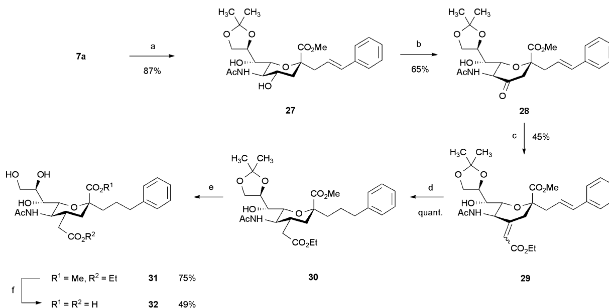
Scheme 6 a) 2,2-Dimethoxy propane, \text{H}^+ (ion exchange), acetone, rt; b) PCC, mol sieve 4 Å, \text{CH}_2\text{Cl}_2 , rt; c) \text{Ph}_3\text{P}=\text{CHCO}_2\text{Et} , THF, rt; d) \text{H}_2 , Pd/C, MeOH, rt; e) \text{H}^+ (ion exchange), \text{H}_2\text{O} , 60 °C; f) 0.1 M NaOH, \text{H}_2\text{O} , rt.
