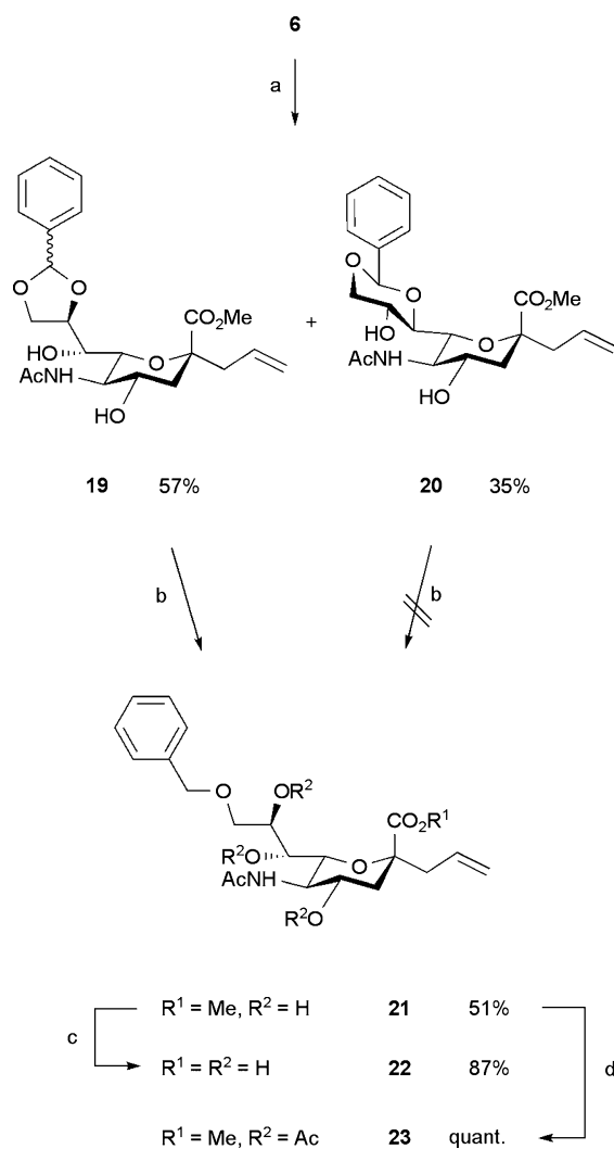
Scheme 4 a) BADMA, pTSA, MeCN, 0 °C; b) BH 3 -Me 3 N, AlCl 3 , THF, H 2 O, rt; c) 0.1 M NaOH, H 2 O, rt; d) Ac 2 O, pyridine.
